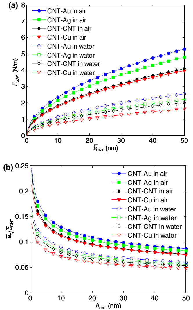
Fig. 3. van der Waals force F_{\text{vdW}} and normalized nanoscale contact width as functions of CNT radius b_{\text{CNT}} . (a) Limiting cases of dry air and water for F_{\text{vdW}} at various CNT contact arrangements. The force is weaker in the presence of water. (b) Limiting cases for the normalized CNT contact width considering elastic, radial CNT deformation. Values near the middle of the limits are used for estimations in this study.
